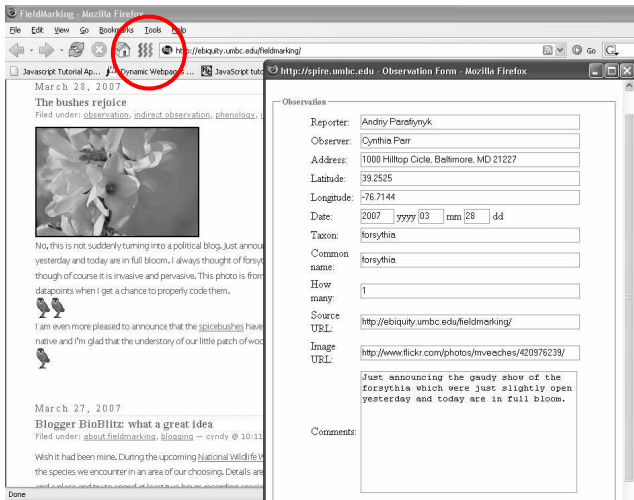
Figure 3. SPOTter form. All fields are optional. Link to blog post is shown with owl icon. Button for launching is shown in red circle
