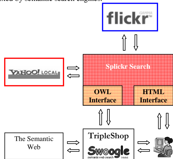
Figure 2 Splickr architecture. For our current purpose, the most relevant parts of the semantic web (lower left corner) are the ETHAN and SpireEcoConcepts ontologies and instance data.
